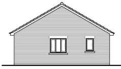
West Elevation
