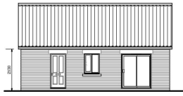
South Elevation
